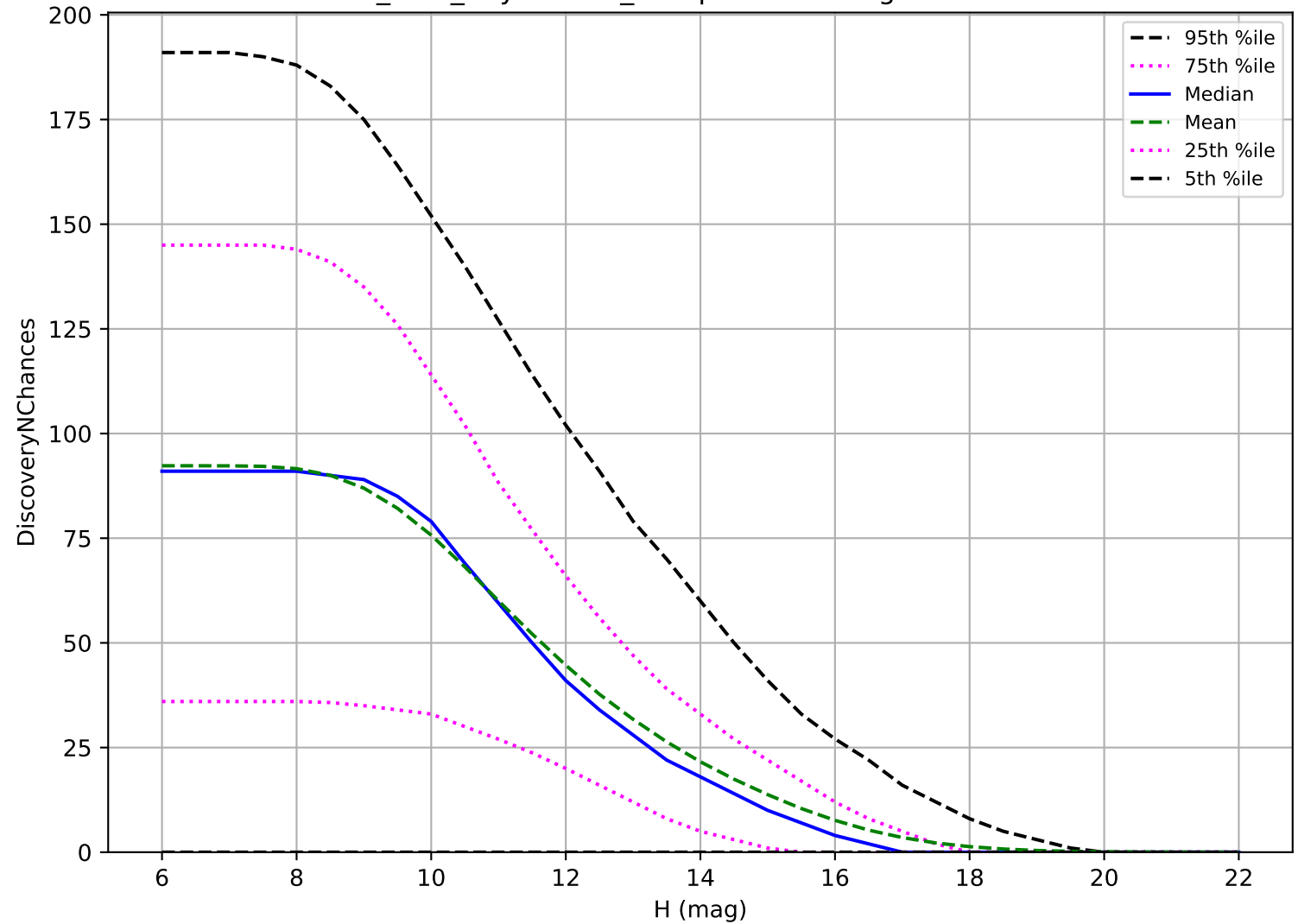
baseline_v2.1_10yrs: OCC_r5 3 pairs in 15 nights detection loss
