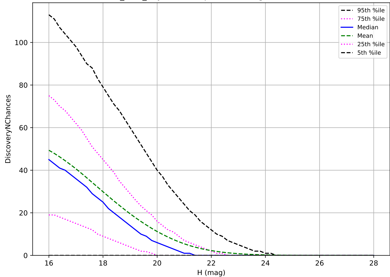
baseline_v2.1_10yrs: NEO 3 pairs in 15 nights detection loss
