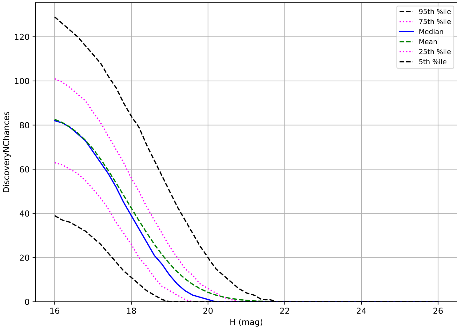
baseline_v2.1_10yrs: MBA 3 pairs in 15 nights detection loss
