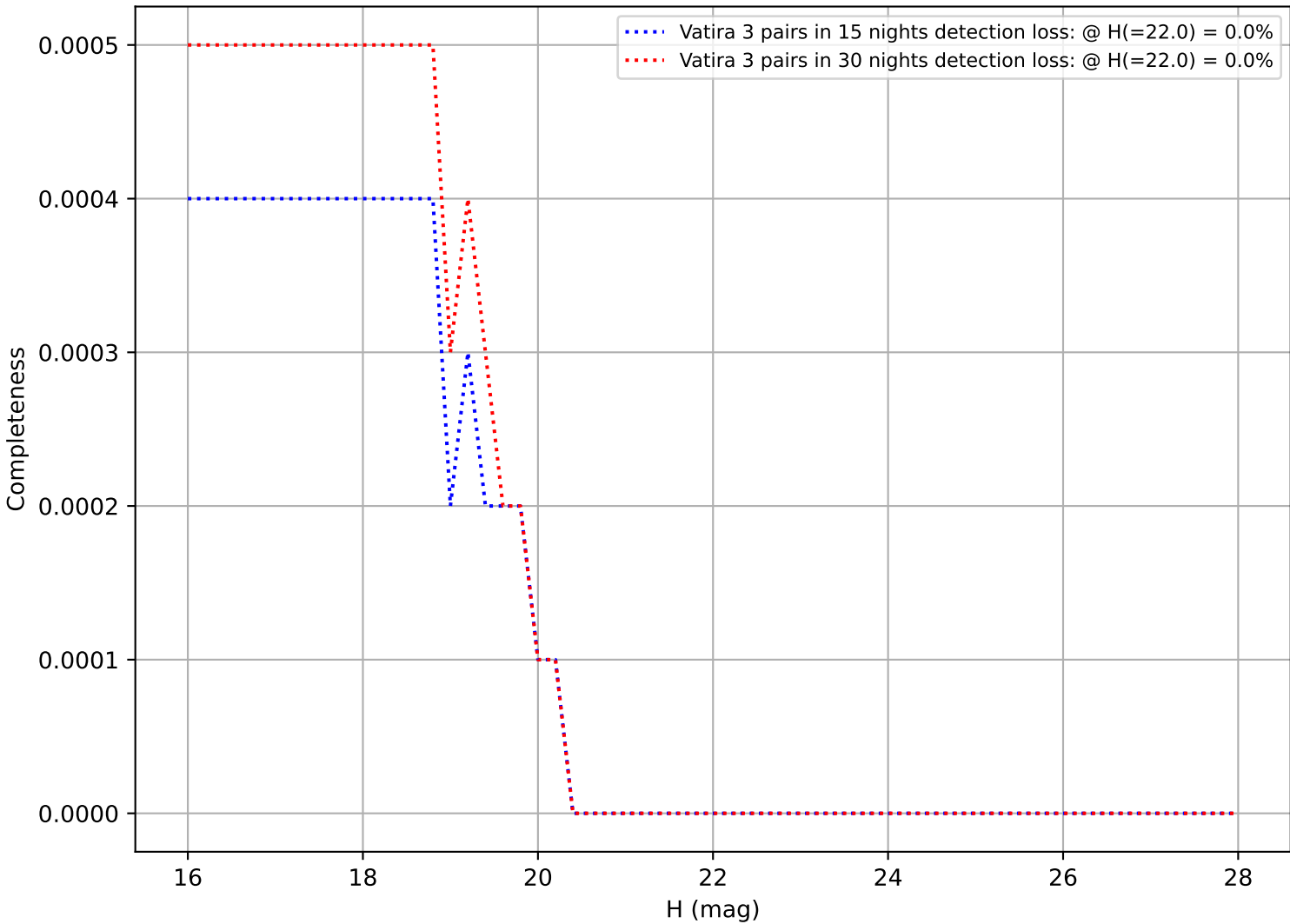
baseline_v2.1_10yrs: DifferentialCompleteness
