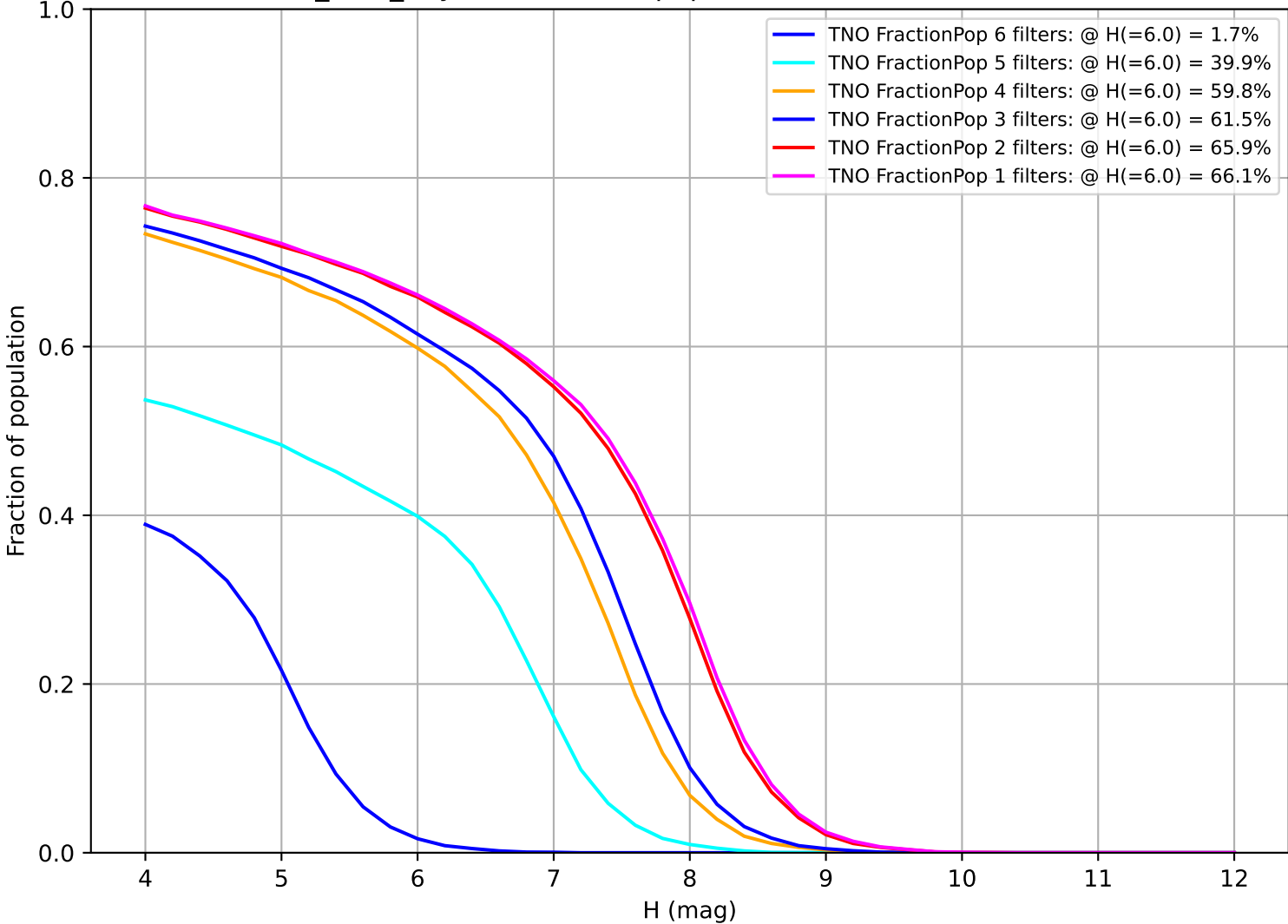
baseline_v2.1_10yrs: Fraction of population with colors in X filters TNO
