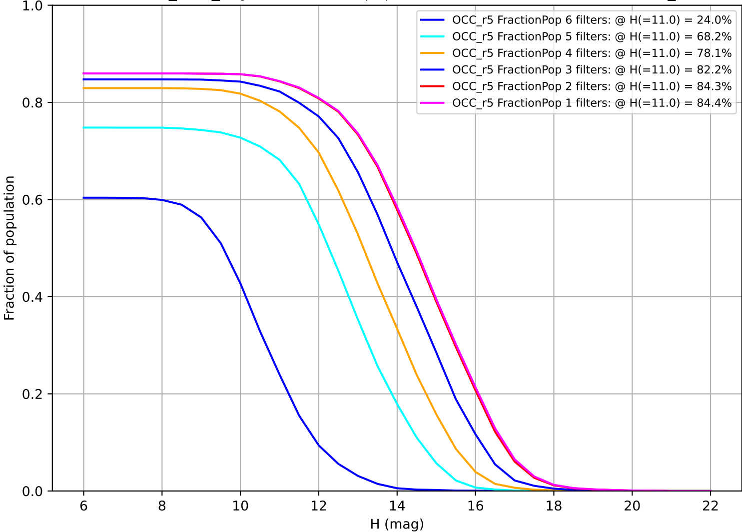
baseline_v2.1_10yrs: Fraction of population with colors in X filters OCC_r5
