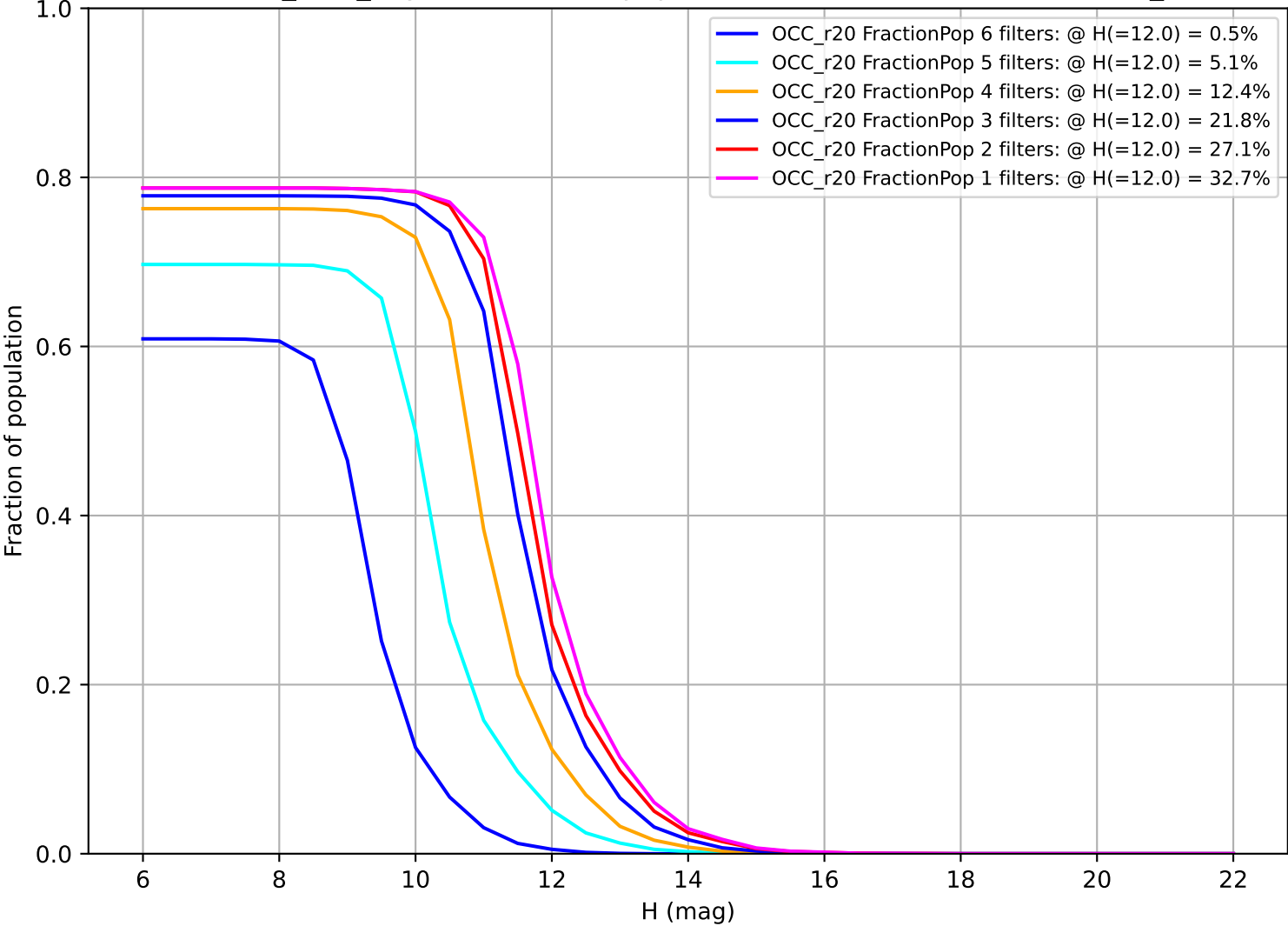
baseline_v2.1_10yrs: Fraction of population with colors in X filters OCC_r20
