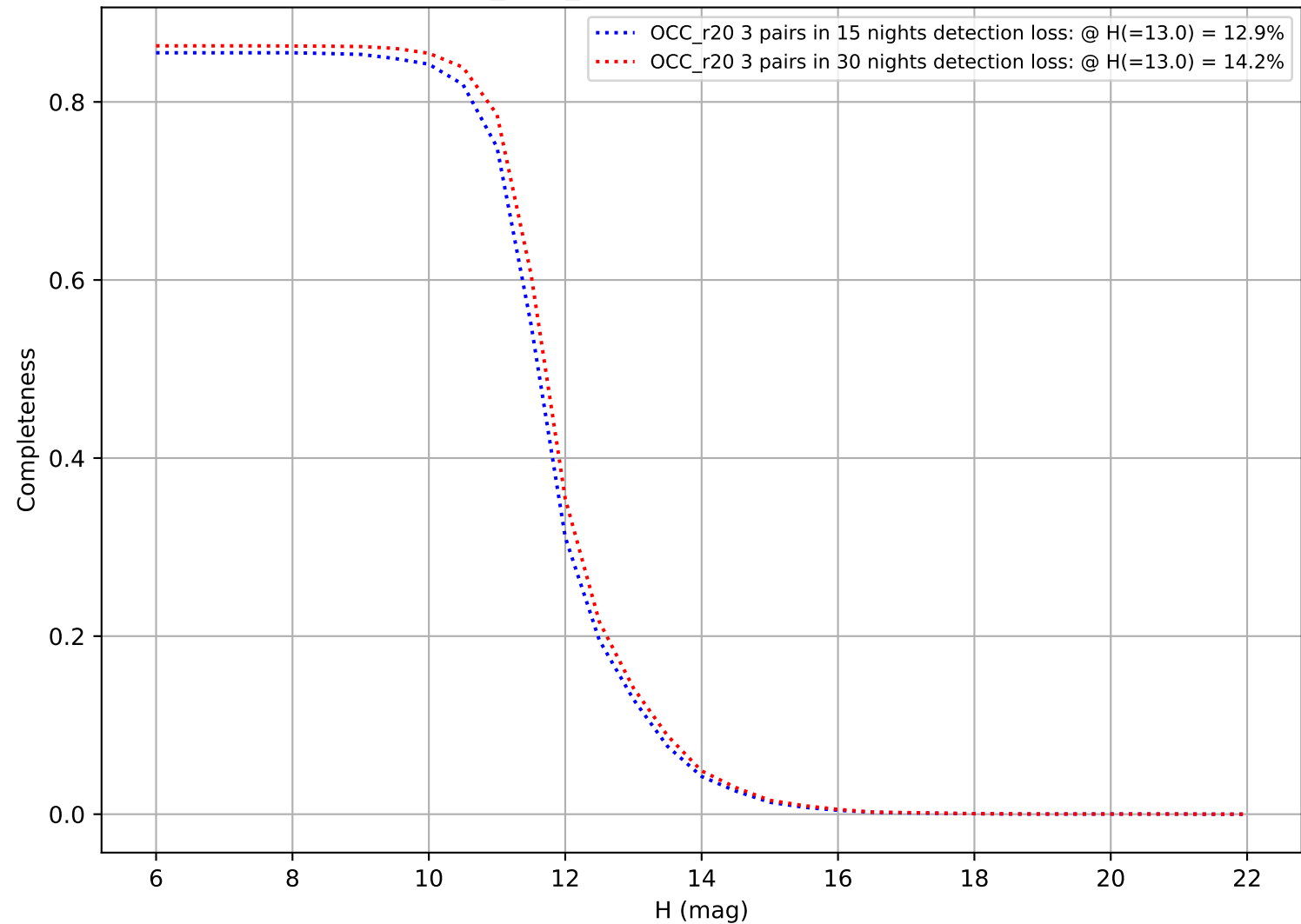
baseline_v2.1_10yrs: DifferentialCompleteness
