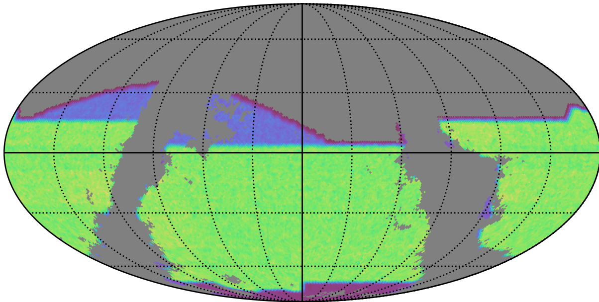
baseline_v2.1_10yrs gri band non-DD: riz_exposure_time_year8
