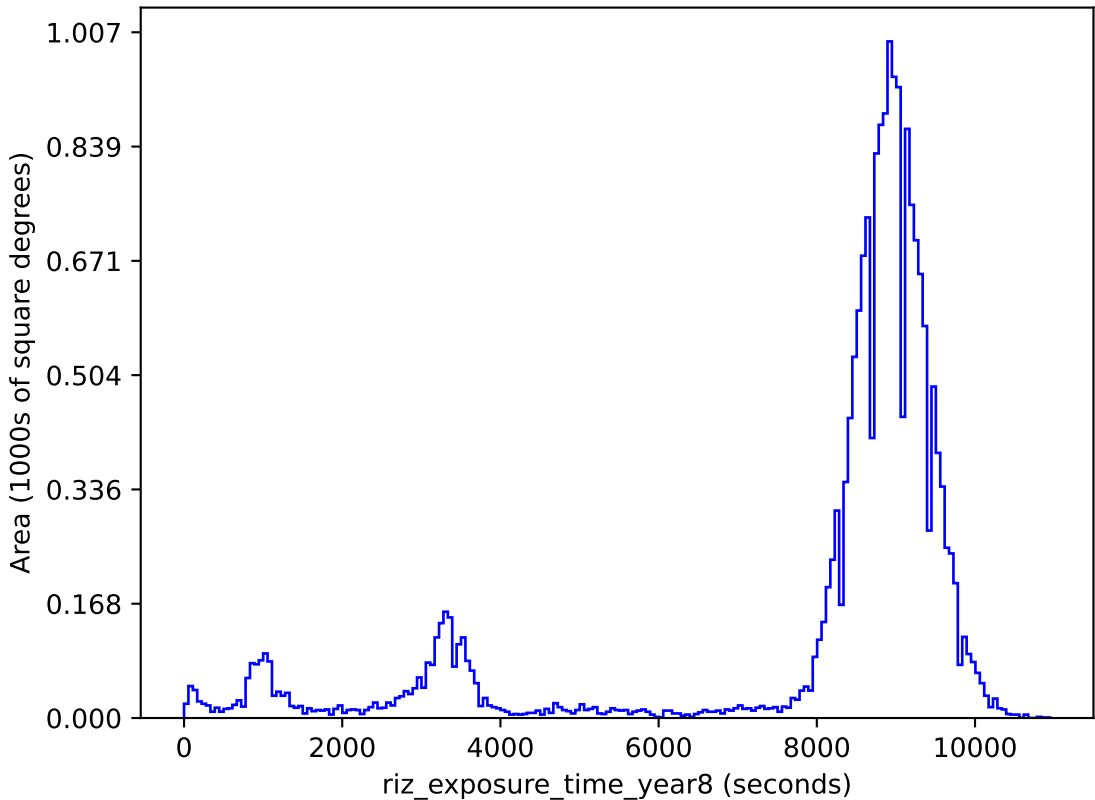
baseline_v2.1_10yrs gri band non-DD: riz_exposure_time_year8
