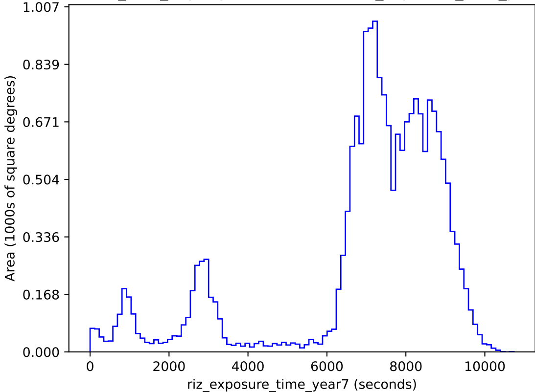
baseline_v2.1_10yrs gri band non-DD: riz_exposure_time_year7
