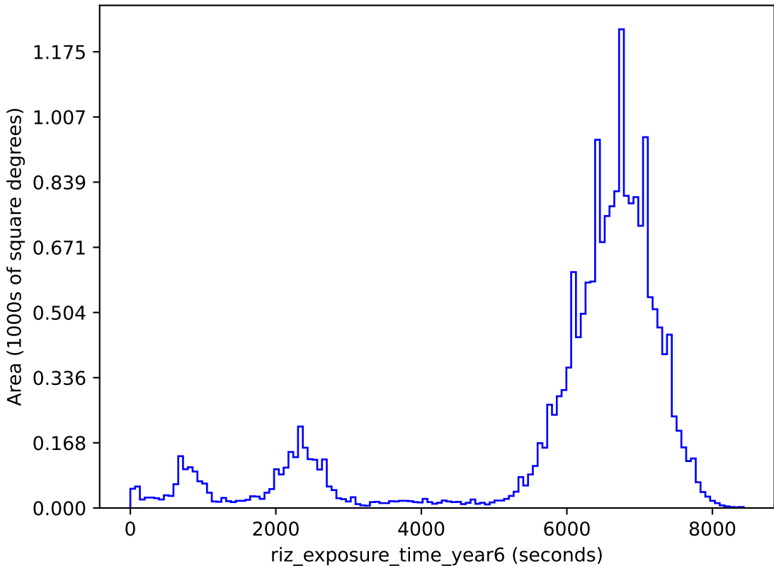
baseline_v2.1_10yrs gri band non-DD: riz_exposure_time_year6
