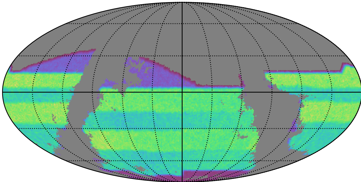
baseline_v2.1_10yrs gri band non-DD: riz_exposure_time_year5
