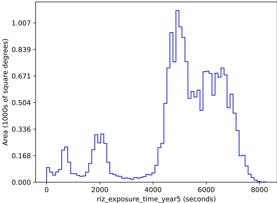
baseline_v2.1_10yrs gri band non-DD: riz_exposure_time_year5
