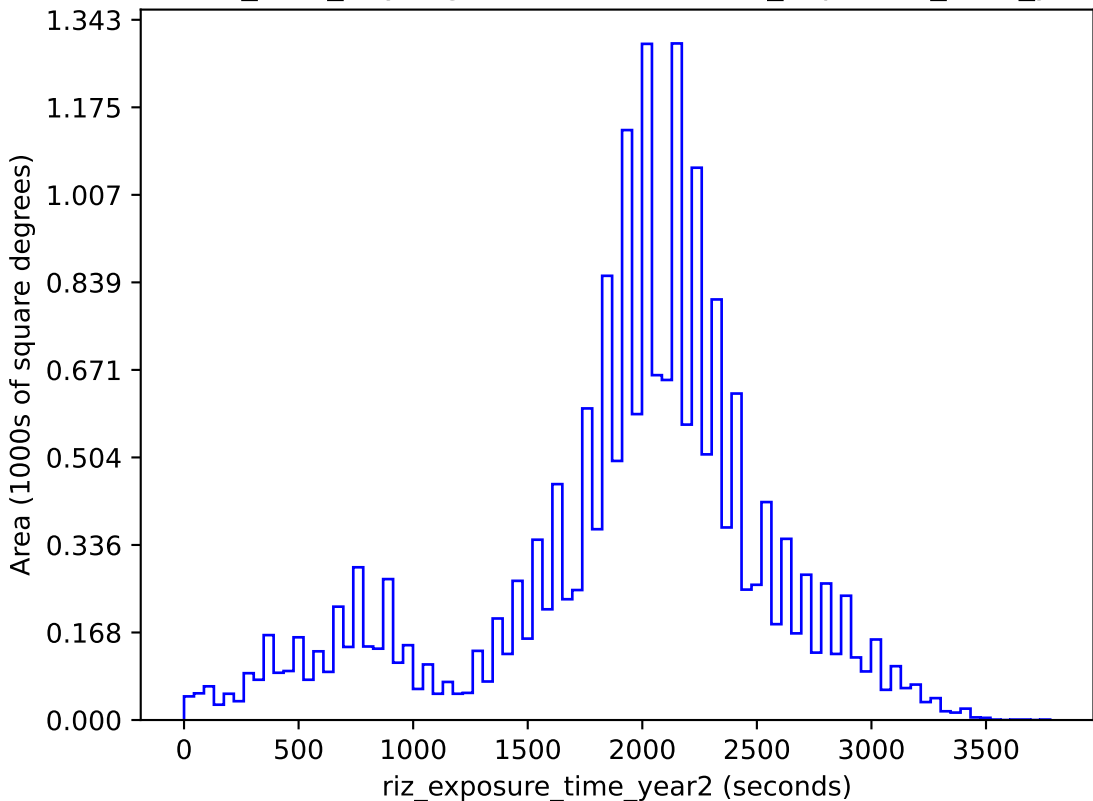
baseline_v2.1_10yrs gri band non-DD: riz_exposure_time_year2
