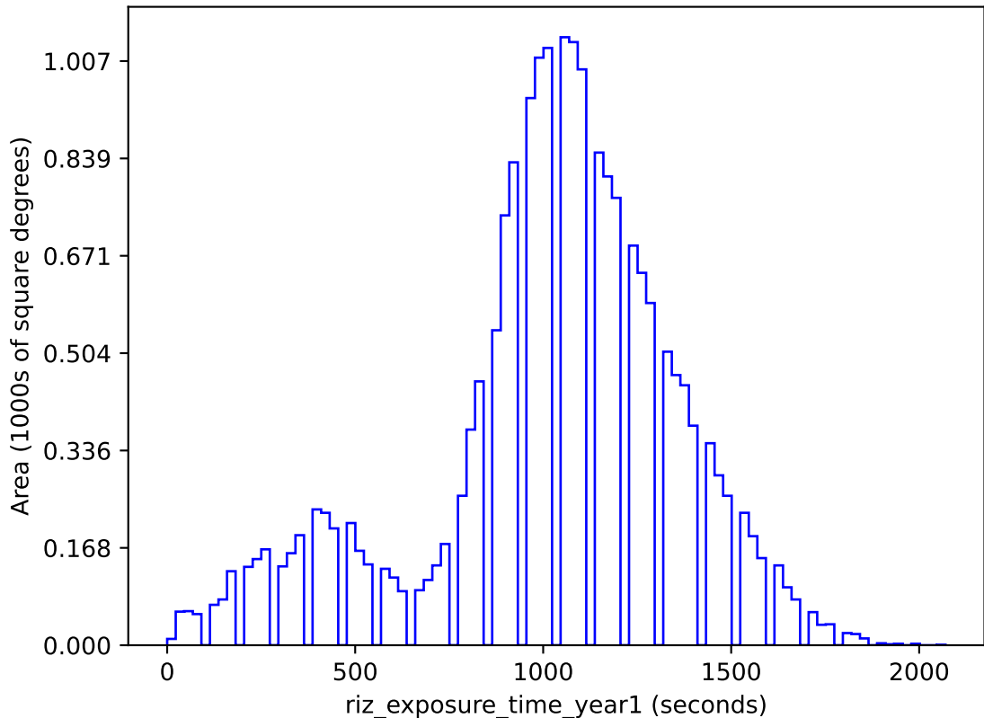
baseline_v2.1_10yrs gri band non-DD: riz_exposure_time_year1
