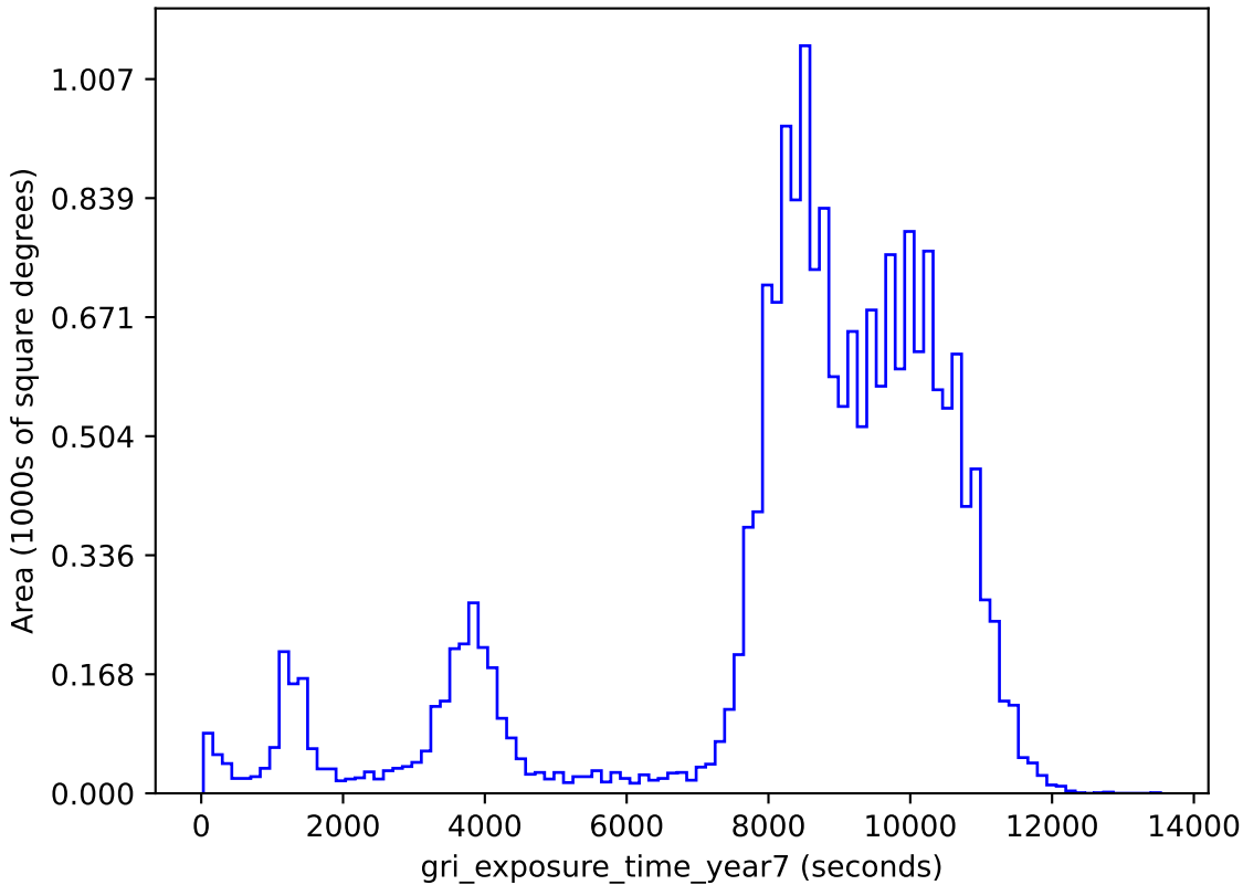
baseline_v2.1_10yrs gri band non-DD: gri_exposure_time_year7
