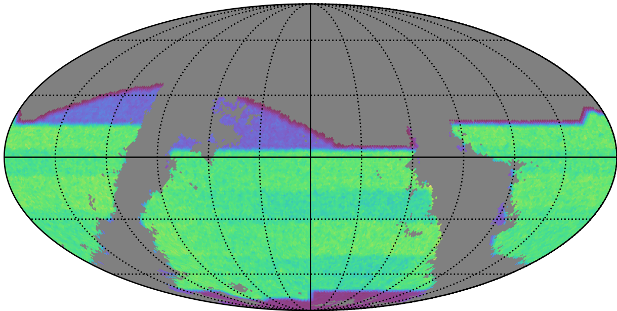
baseline_v2.1_10yrs gri band non-DD: gri_exposure_time_year6
