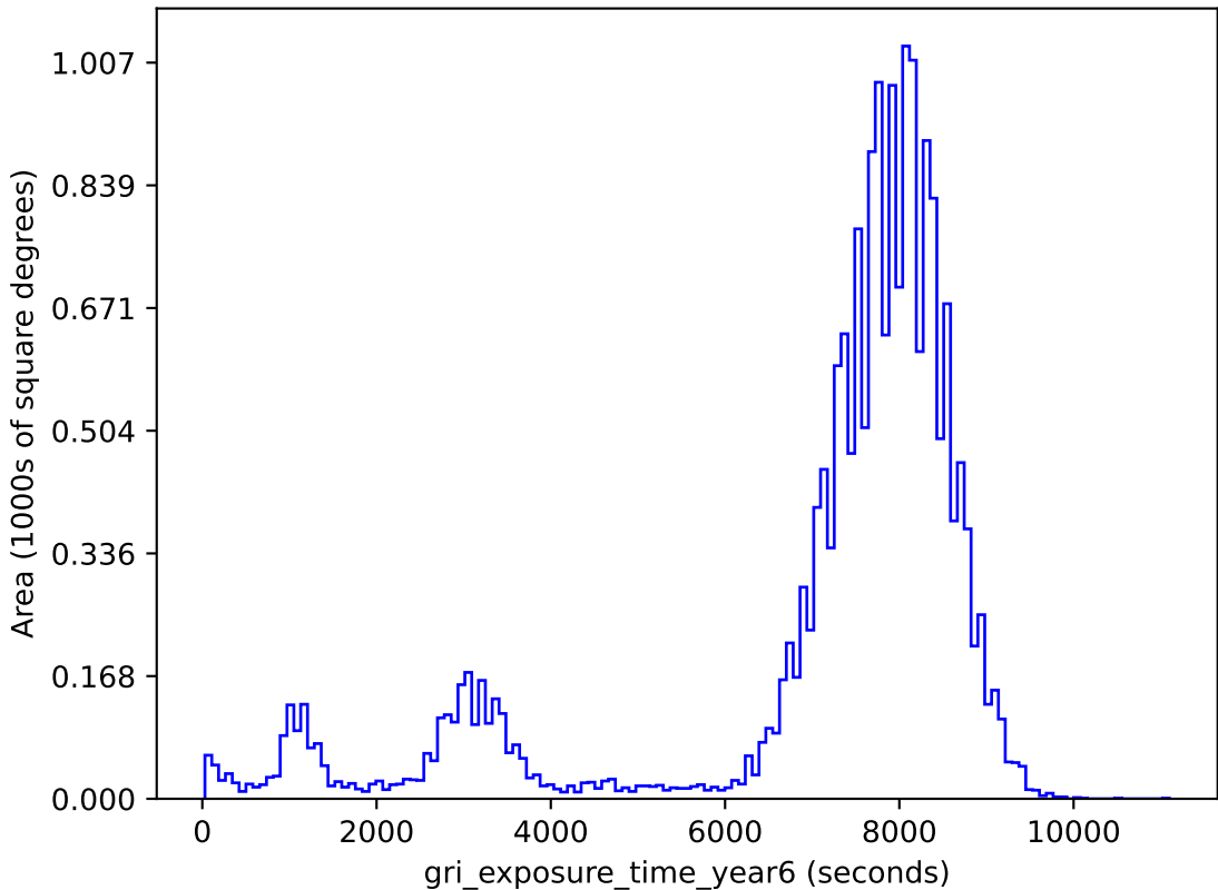
baseline_v2.1_10yrs gri band non-DD: gri_exposure_time_year6
