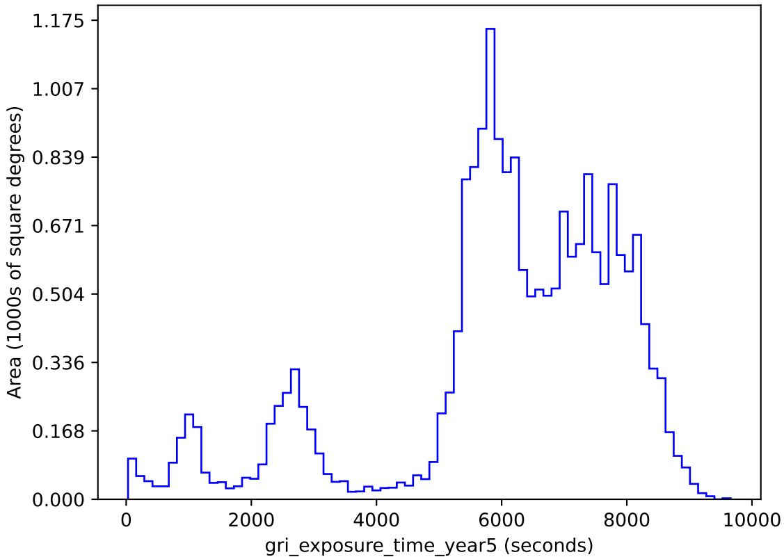
baseline_v2.1_10yrs gri band non-DD: gri_exposure_time_year5
