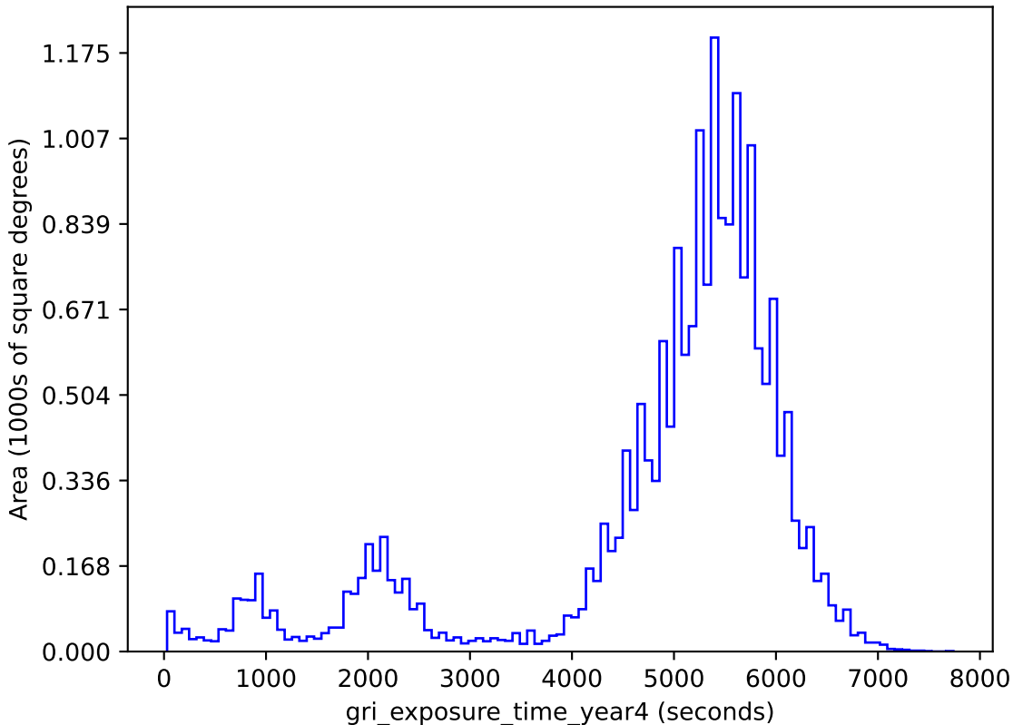
baseline_v2.1_10yrs gri band non-DD: gri_exposure_time_year4
