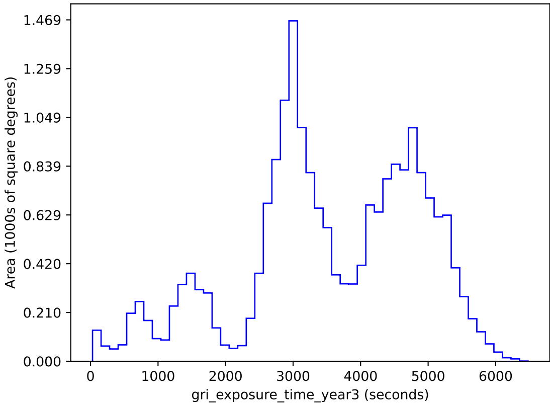
baseline_v2.1_10yrs gri band non-DD: gri_exposure_time_year3
