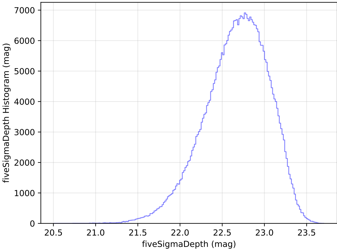
baseline_v2.1_10yrs z: fiveSigmaDepth Histogram
