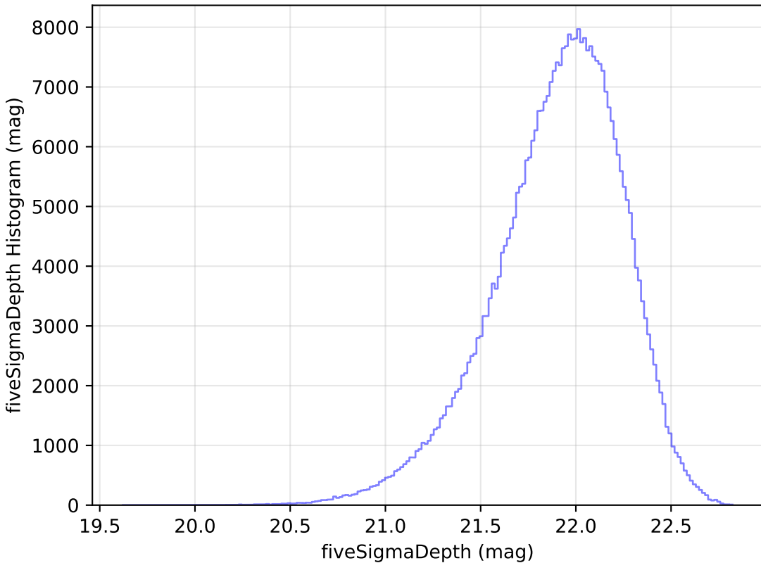
baseline_v2.1_10yrs y: fiveSigmaDepth Histogram
