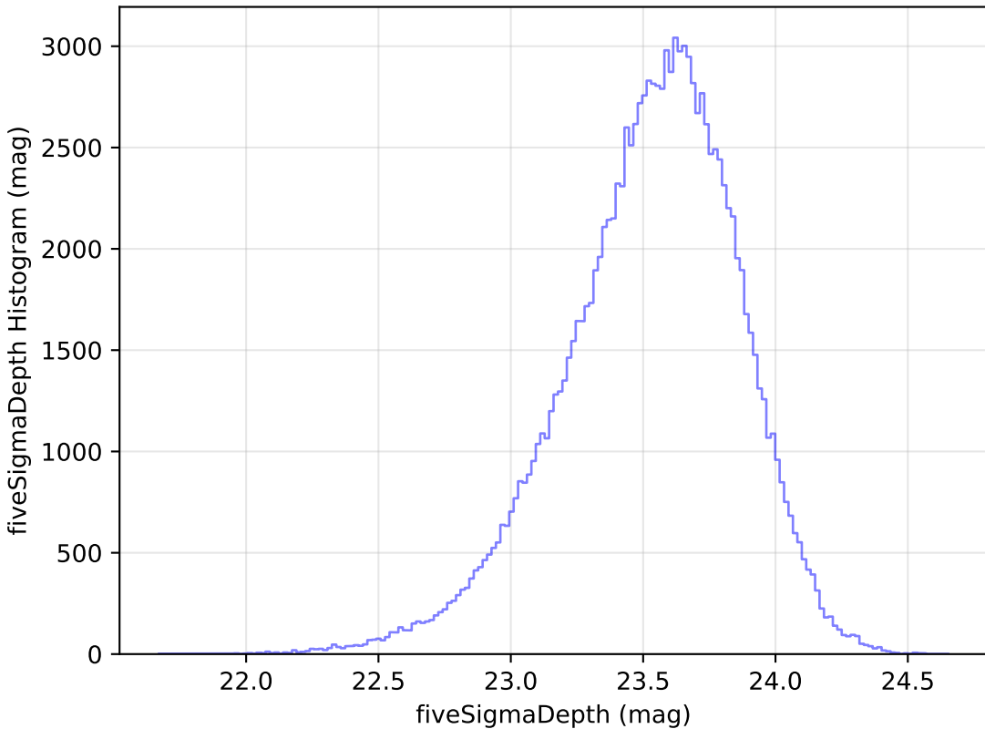
baseline_v2.1_10yrs u: fiveSigmaDepth Histogram
