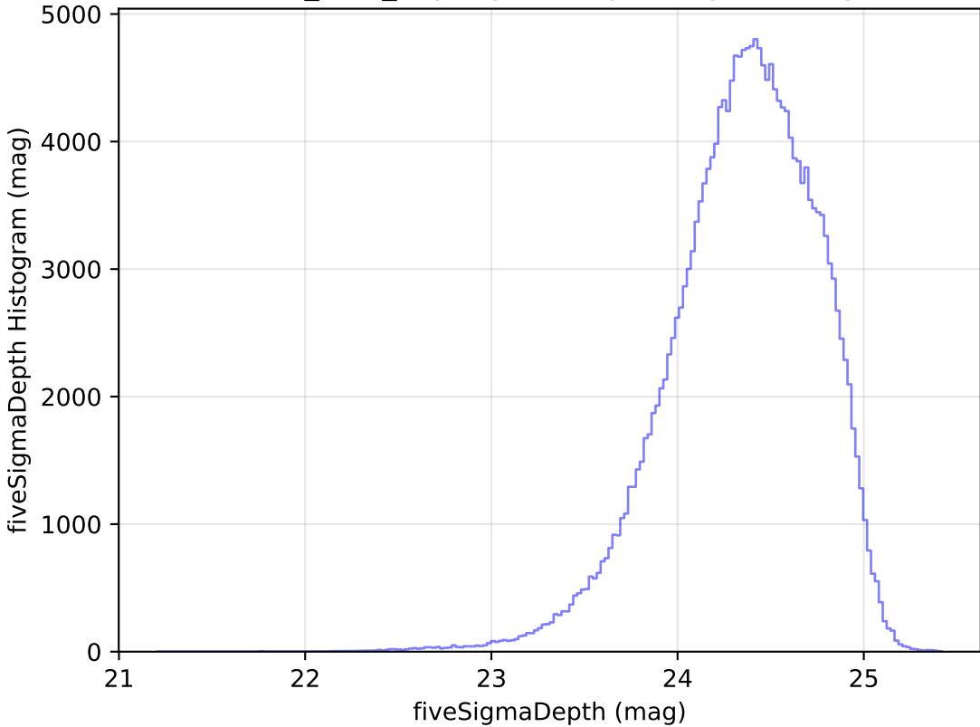
baseline_v2.1_10yrs g: fiveSigmaDepth Histogram
