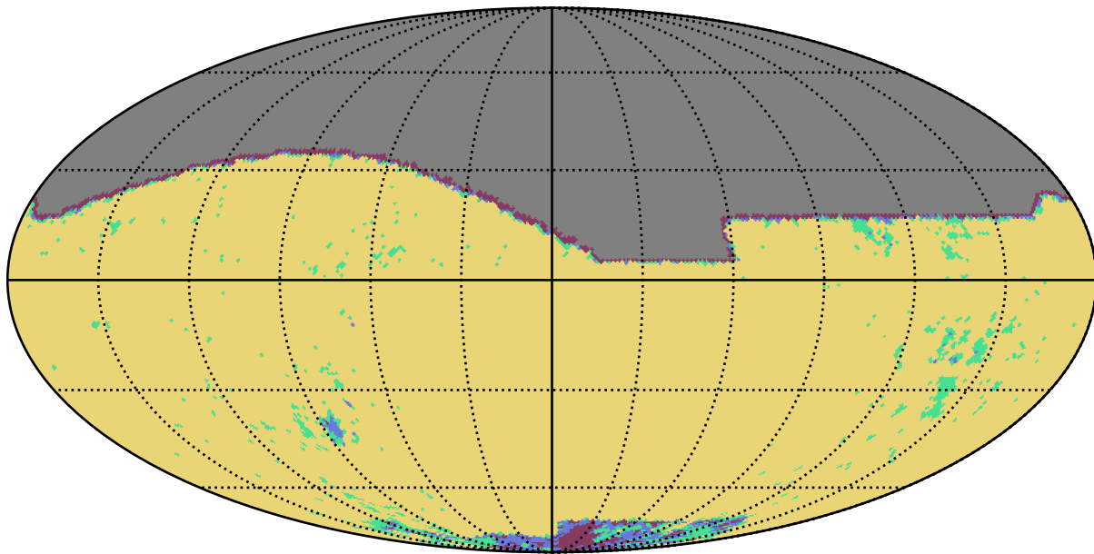
baseline_v2.1_10yrs z band: YearCoverage night
