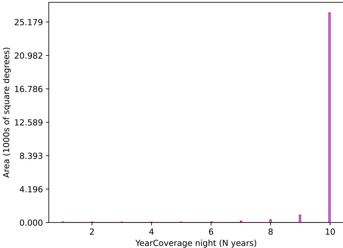
baseline_v2.1_10yrs z band: YearCoverage night
