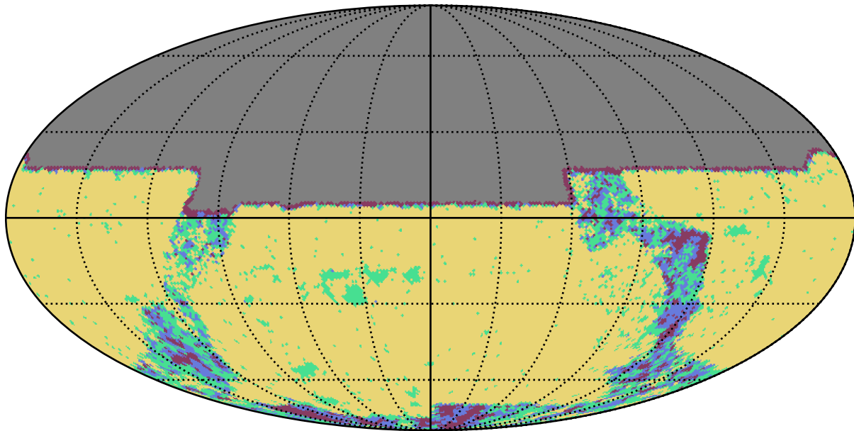
baseline_v2.1_10yrs u band: YearCoverage night
