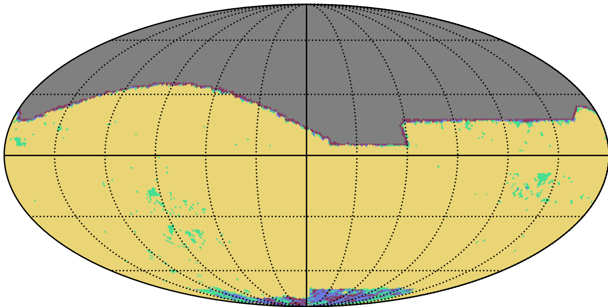
baseline_v2.1_10yrs r band: YearCoverage night
