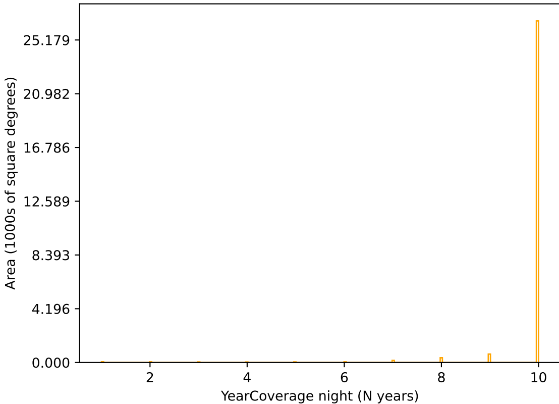
baseline_v2.1_10yrs r band: YearCoverage night
