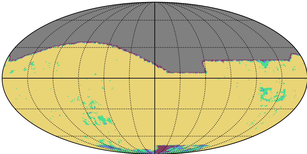
baseline_v2.1_10yrs i band: YearCoverage night
