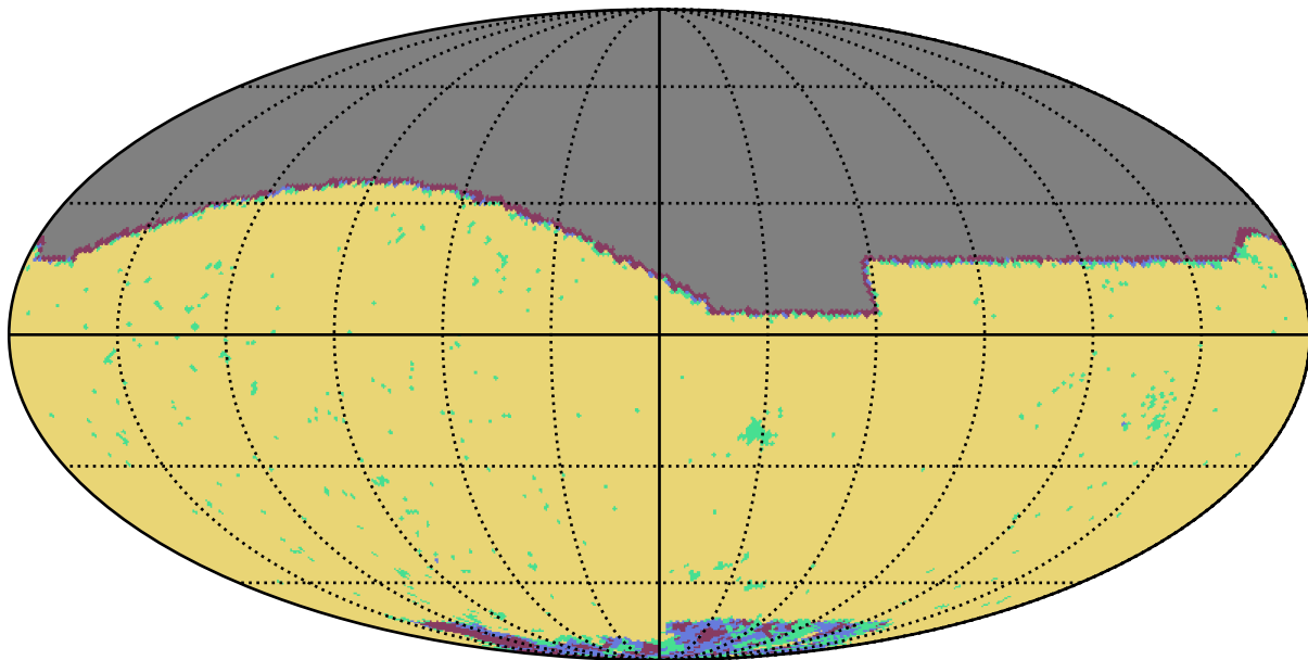
baseline_v2.1_10yrs g band: YearCoverage night
