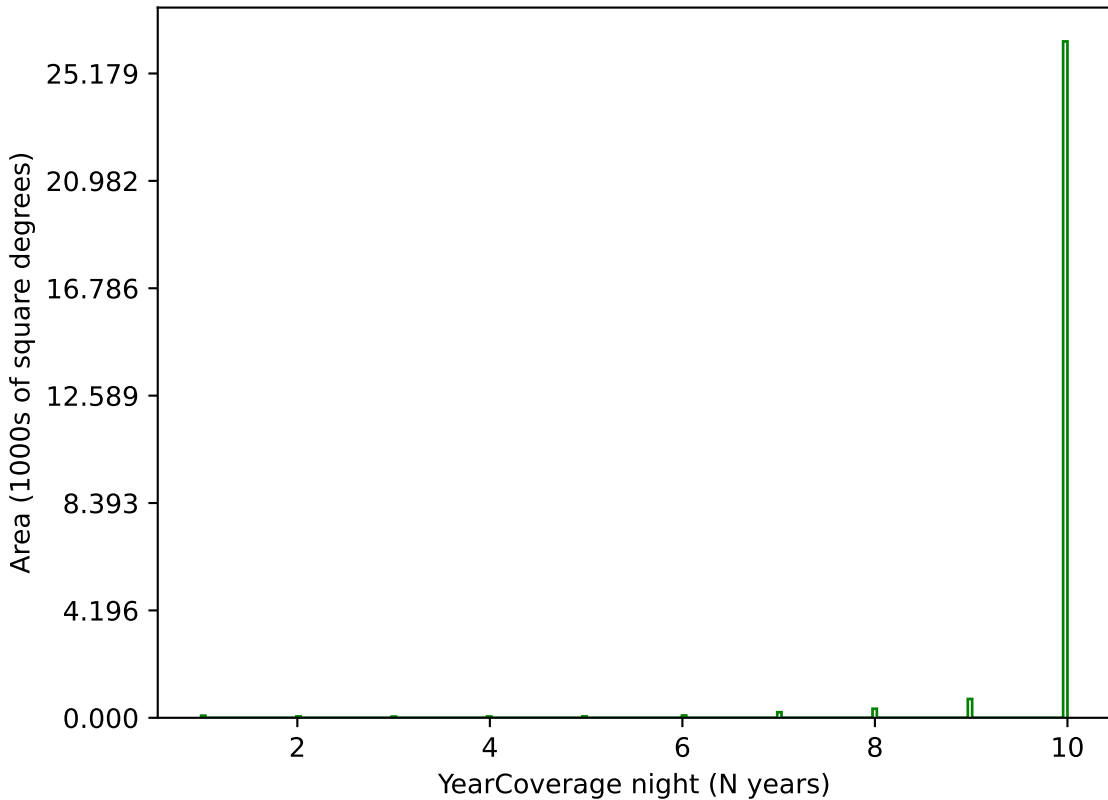
baseline_v2.1_10yrs g band: YearCoverage night
