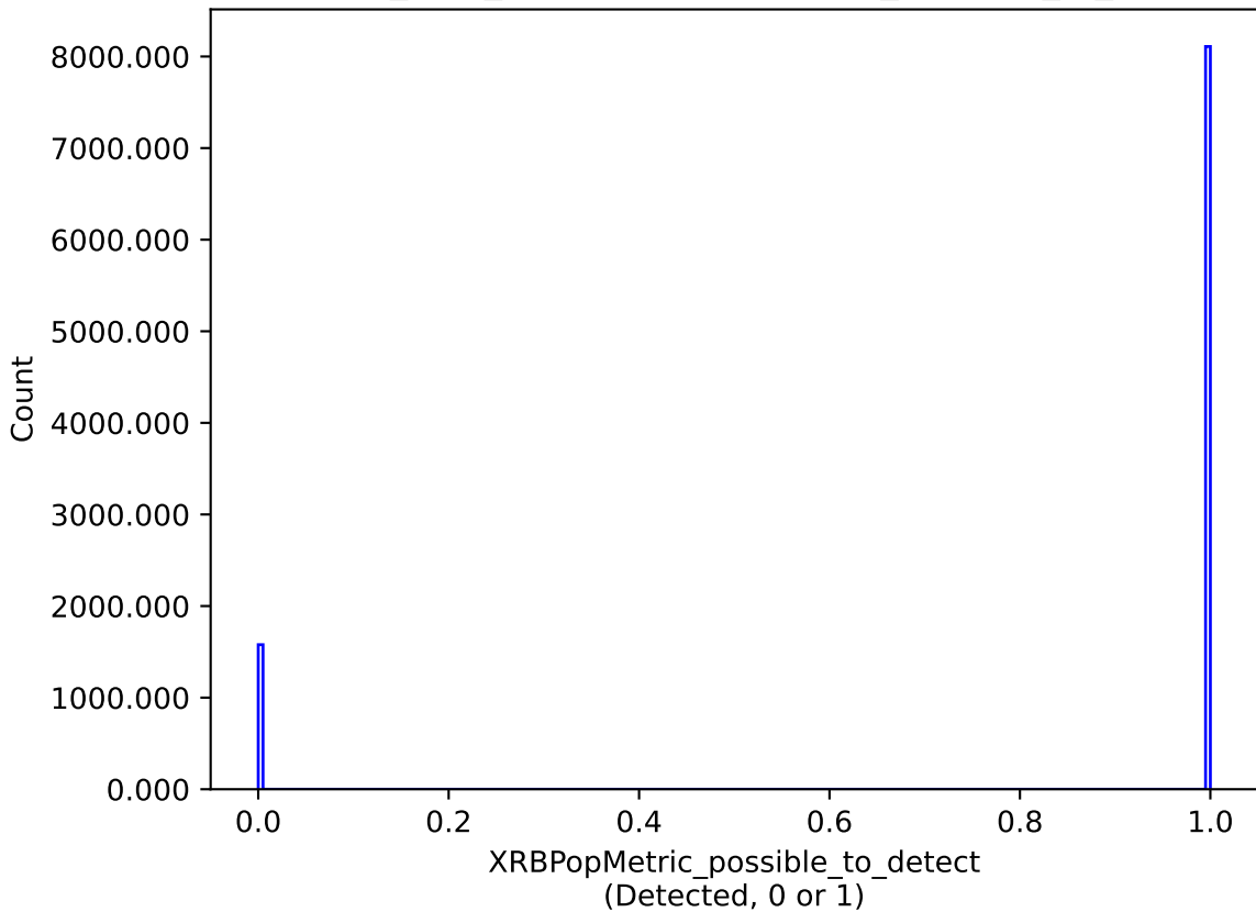
baseline_v2.1_10yrs : XRBPoMetric_possible_to_detect
