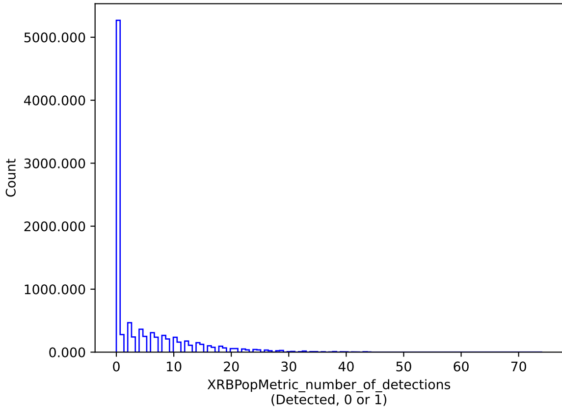
baseline_v2.1_10yrs : XRBPopMetric_number_of_detections
