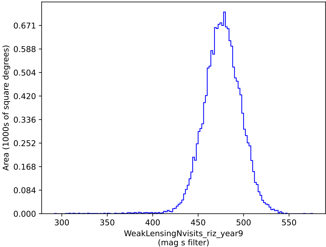
baseline_v2.1_10yrs gri band non-DD: WeakLensingNvisits_riz_year9
