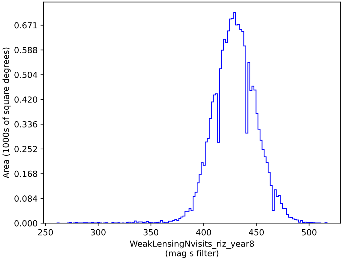
baseline_v2.1_10yrs gri band non-DD: WeakLensingNvisits_riz_year8
