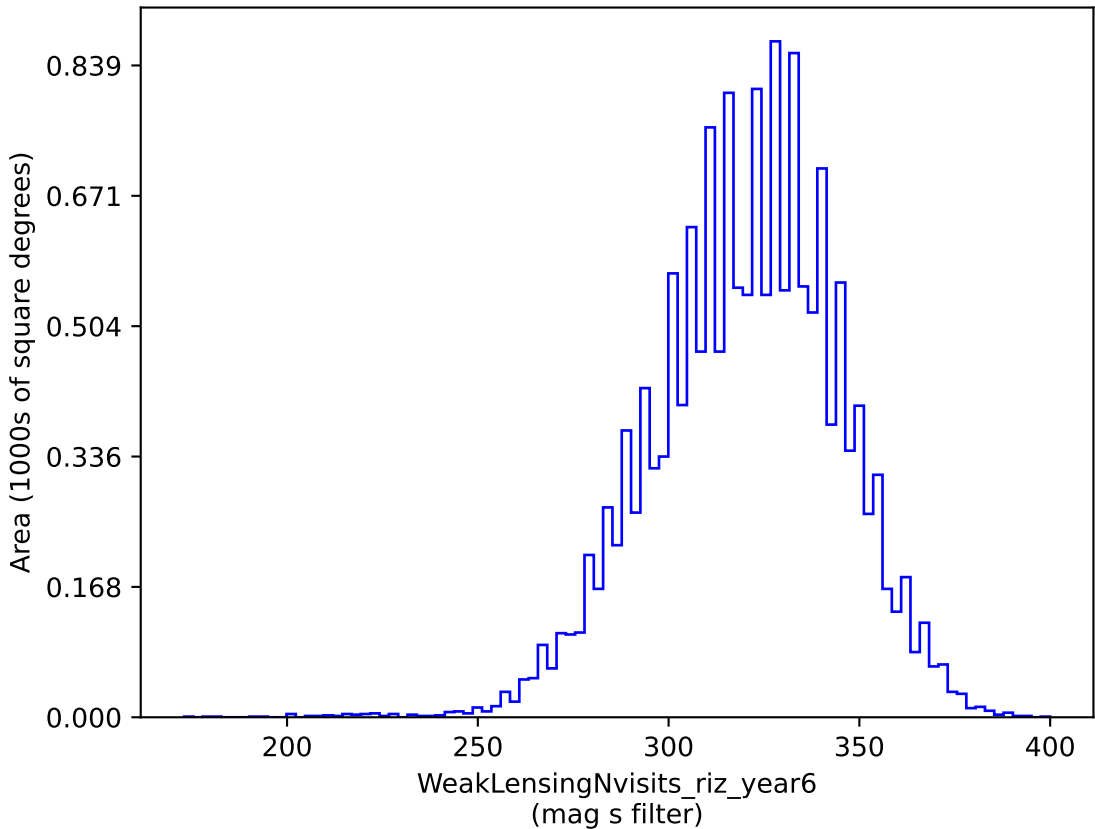
baseline_v2.1_10yrs gri band non-DD: WeakLensingNvisits_riz_year6
