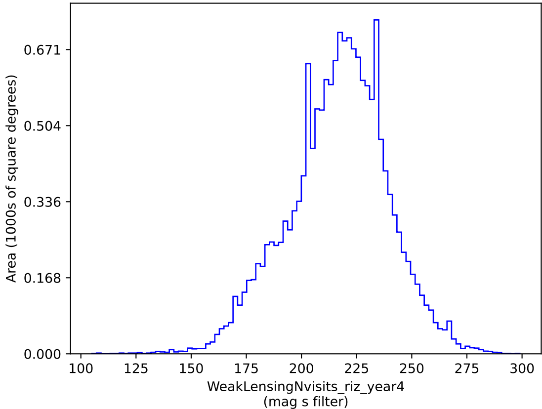
baseline_v2.1_10yrs gri band non-DD: WeakLensingNvisits_riz_year4
