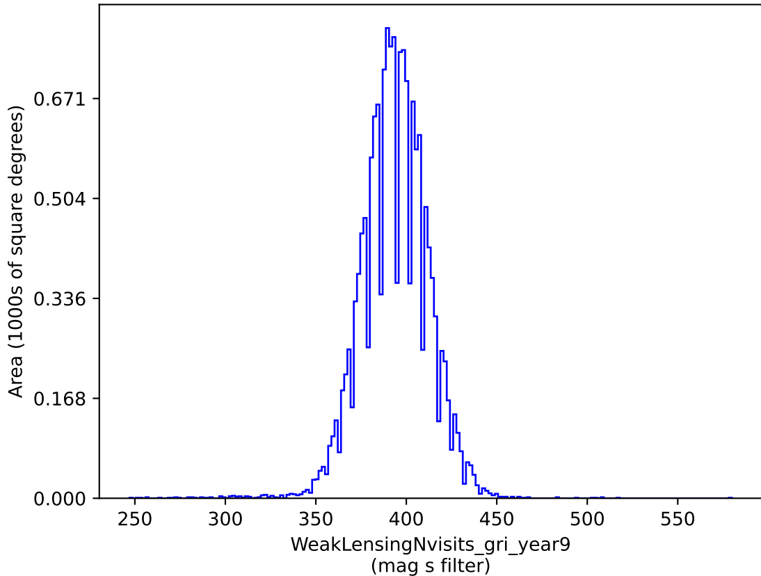
baseline_v2.1_10yrs gri band non-DD: WeakLensingNvisits_gri_year9
