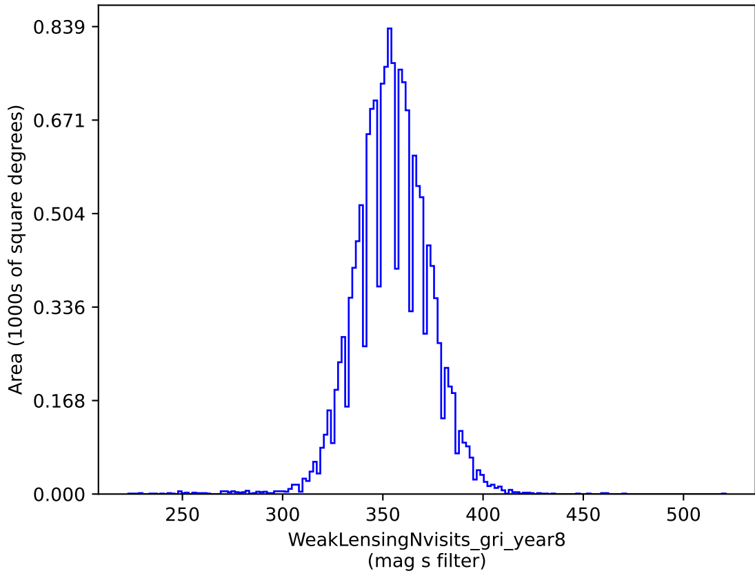
baseline_v2.1_10yrs gri band non-DD: WeakLensingNvisits_gri_year8
