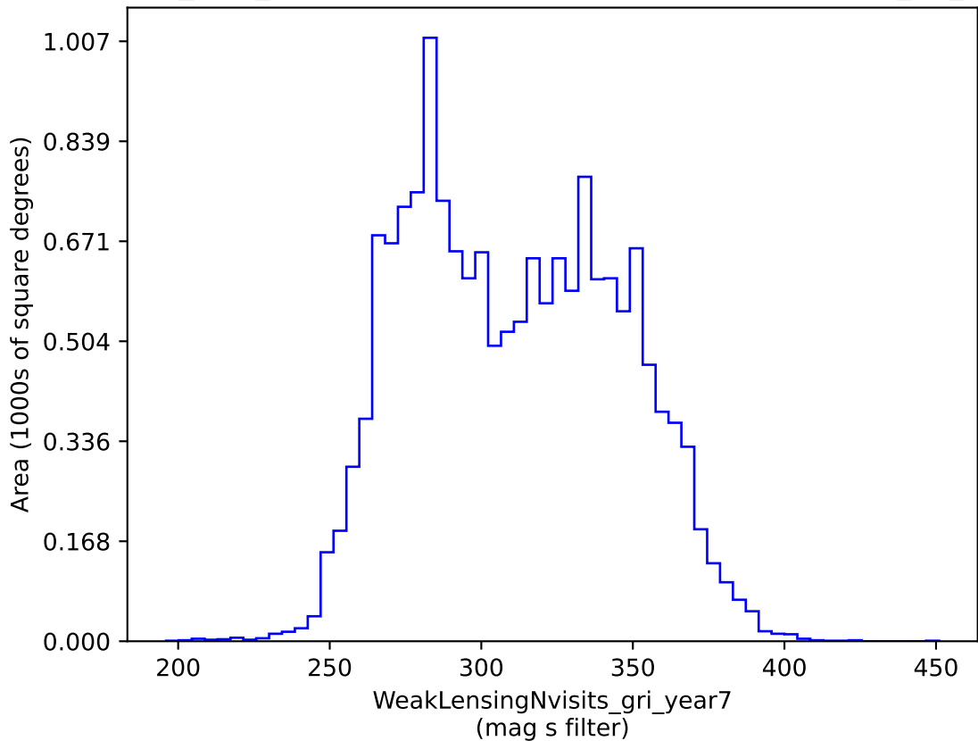
baseline_v2.1_10yrs gri band non-DD: WeakLensingNvisits_gri_year7
