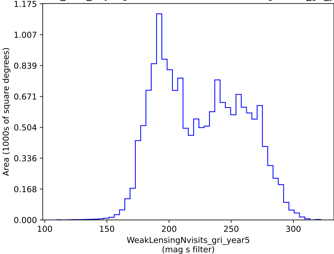
baseline_v2.1_10yrs gri band non-DD: WeakLensingNvisits_gri_year5
