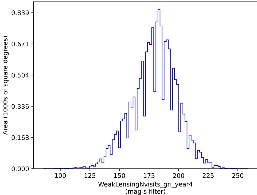
baseline_v2.1_10yrs gri band non-DD: WeakLensingNvisits_gri_year4
