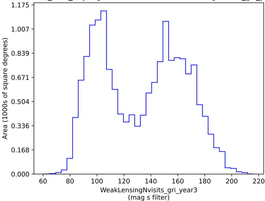
baseline_v2.1_10yrs gri band non-DD: WeakLensingNvisits_gri_year3
