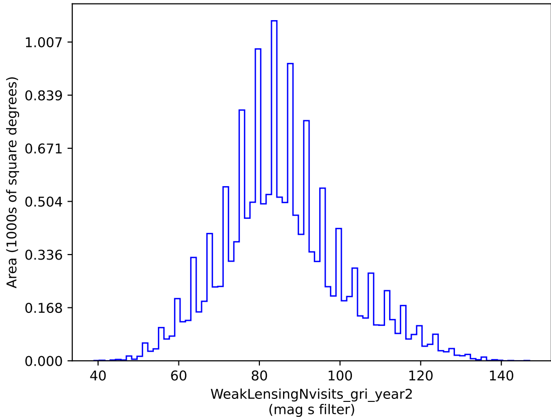
baseline_v2.1_10yrs gri band non-DD: WeakLensingNvisits_gri_year2
