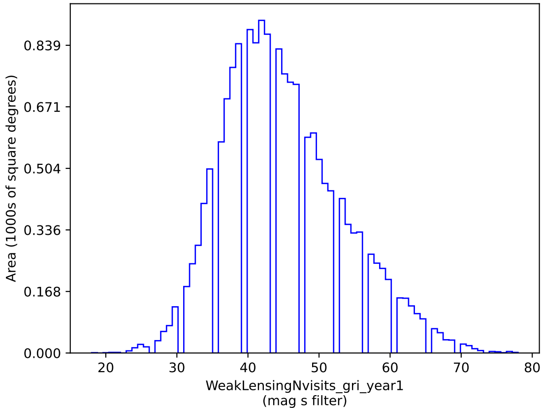
baseline_v2.1_10yrs gri band non-DD: WeakLensingNvisits_gri_year1
