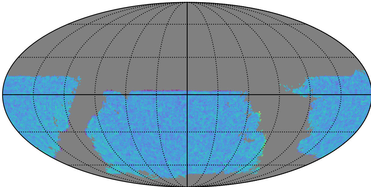
baseline_v2.1_10yrs gri band non-DD: WeakLensingNvisits
