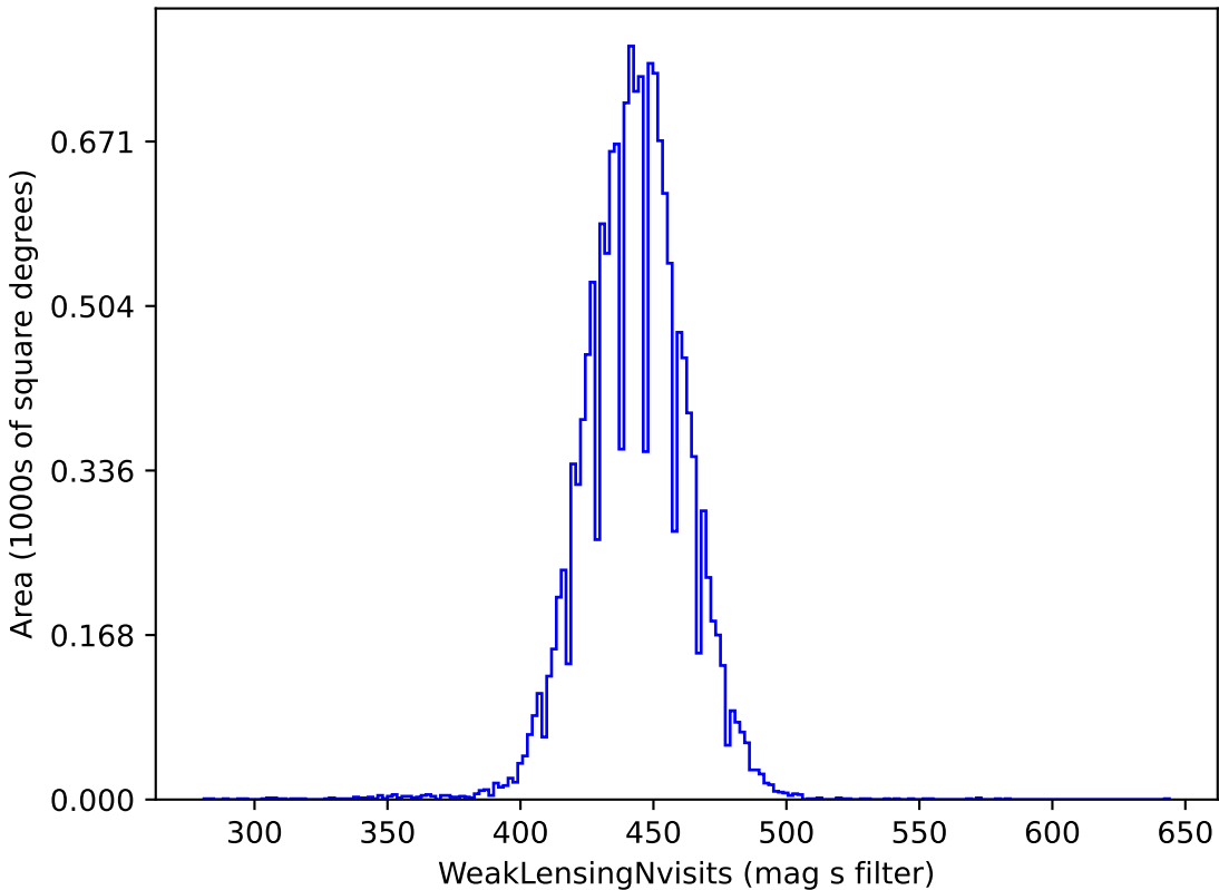
baseline_v2.1_10yrs gri band non-DD: WeakLensingNvisits
